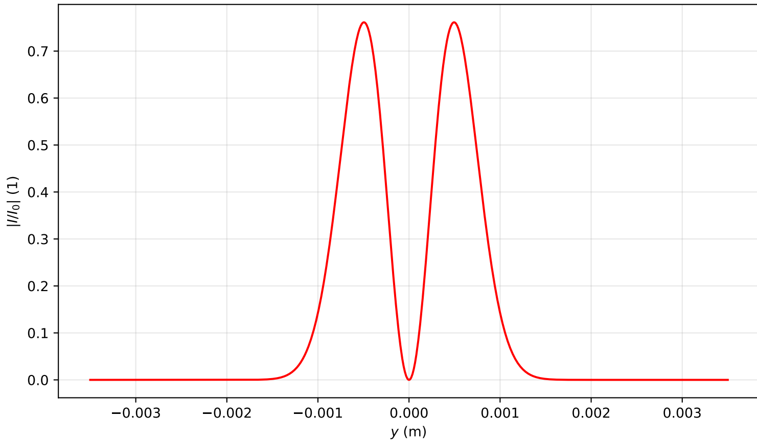
Intensity profile I(x=0, y, z=0.000)/I_0 , P_{in}=4.0P_{cr} , artificial time
